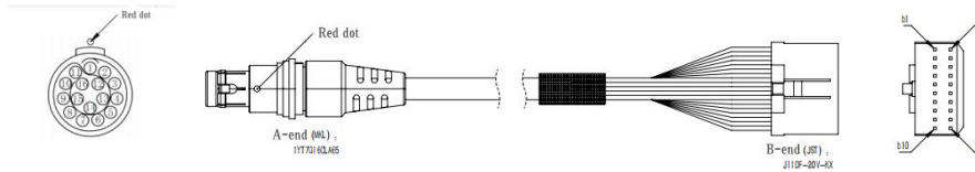
Figure 2-3 16 Pin Airline
