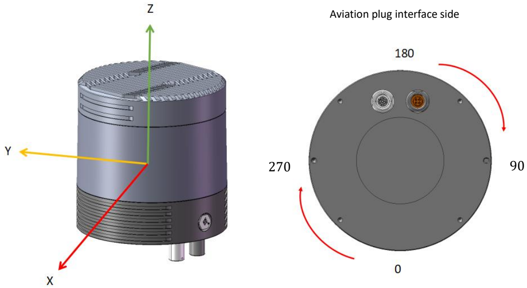
Figure 2-1 LiDAR Coordinate and Rotation Direction
