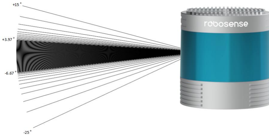
Figure 6-1 RS-Ruby_Plus Vertical Angles
