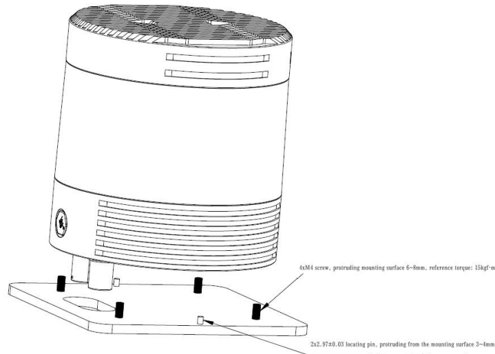
Figure 3-1 LiDAR Mounting Details
