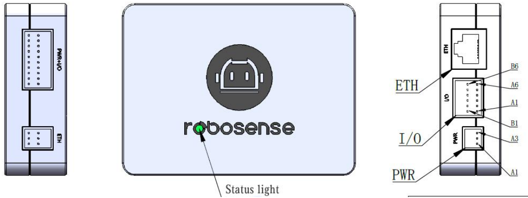
Figure 2-4 Interface Box Schematic
