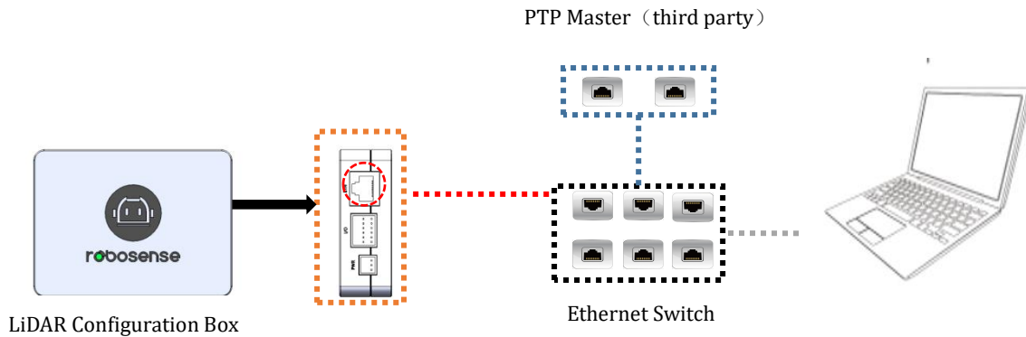
Figure 4-4 PTP Connecting Diagram
