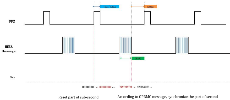
Figure 4-3 GPS Time Synchronization Timing Diagram
